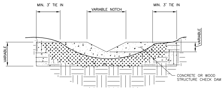
6 TYPICAL STRUCTURAL CHECK DAM CROSS SECTION NOT TO SCALE
