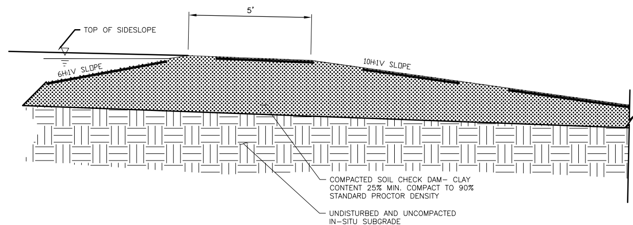
1 TYPICAL EARTHEN CHECK DAM PROFILE NOT TO SCALE
