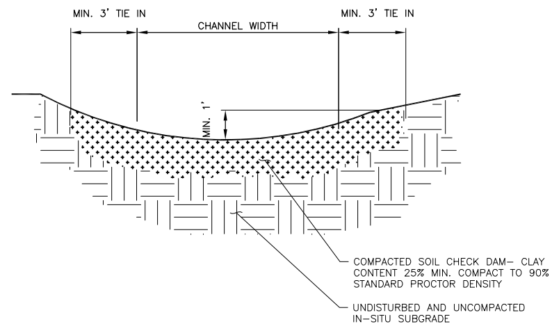
2 TYPICAL EARTHEN CHECK DAM CROSS SECTION NOT TO SCALE
