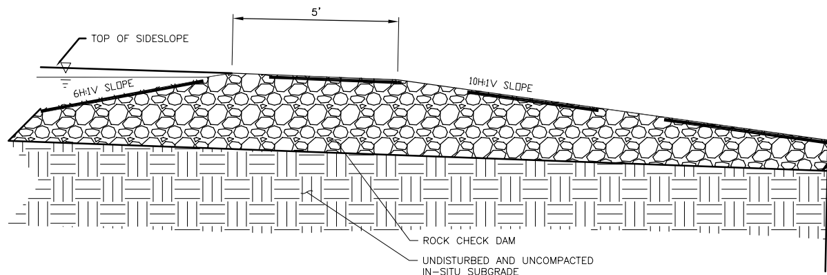
3 TYPICAL ROCK CHECK DAM PROFILE NOT TO SCALE
