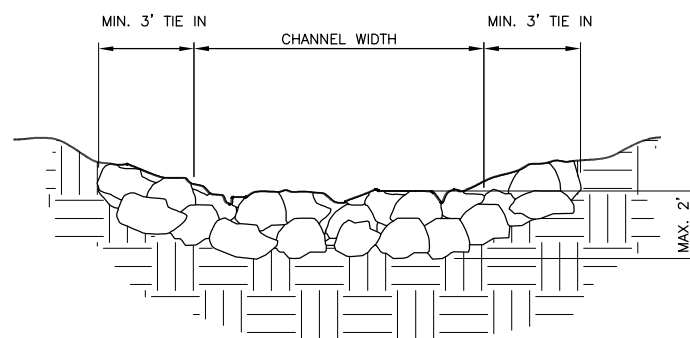
4 TYPICAL ROCK CHECK DAM CROSS SECTION NOT TO SCALE
