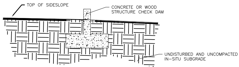
5 TYPICAL STRUCTURAL CHECK DAM PROFILE NOT TO SCALE
